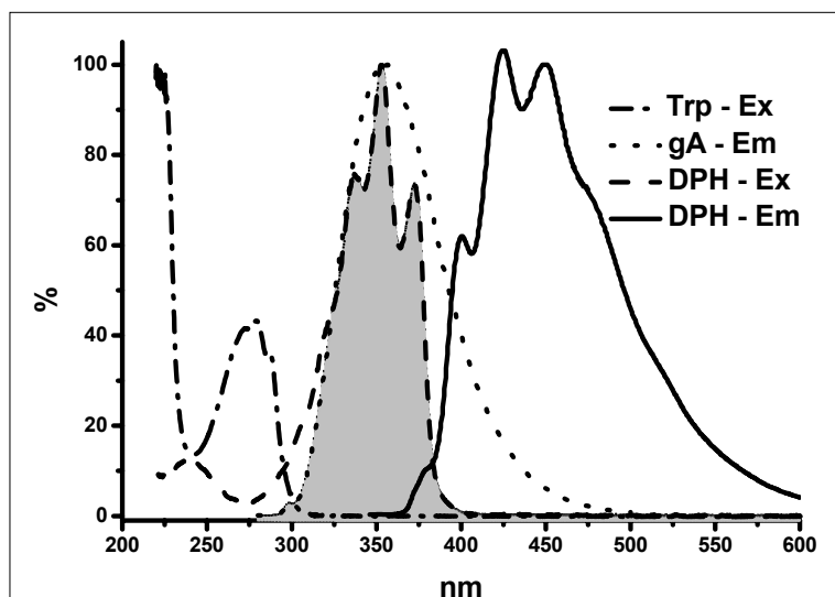
Fig. 1. Normalized absorption and emission spectra of Trp, GA and DPH.
