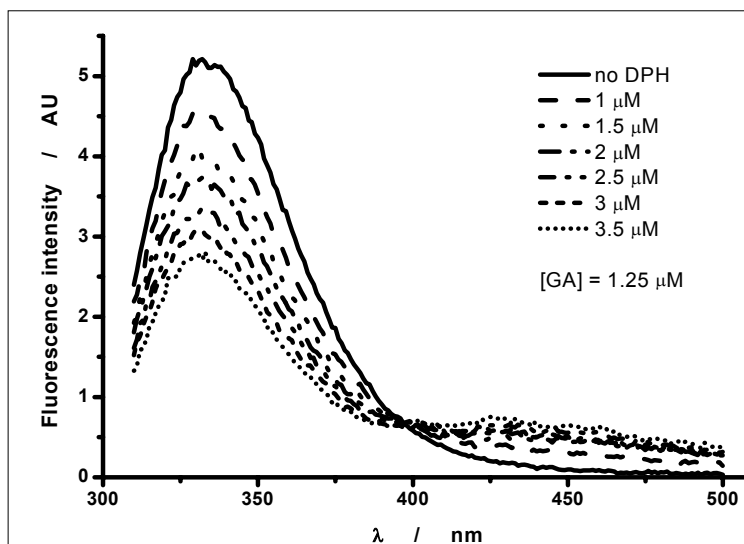
Fig. 2. FRET spectra for various acceptor concentrations recorded on liposomes doped with GA and TMA-DPH.
