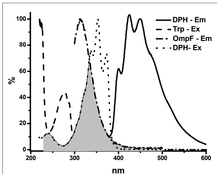
Fig. 4. Normalized absorption and emission spectra of Trp, OmpF and DPH.
