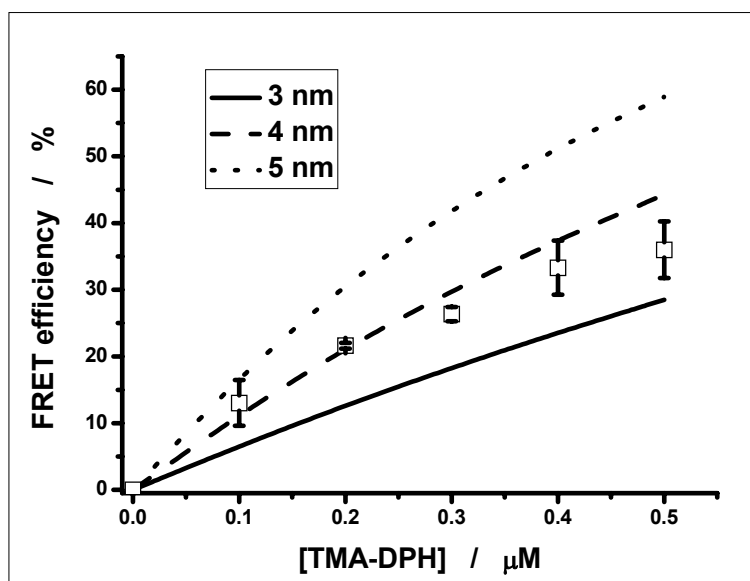
Fig. 8. Simulated FRET efficiency in comparison with experimental data for the OmpF experiments.
