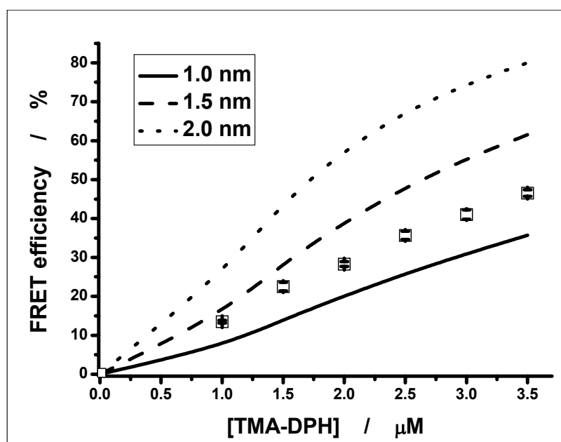
Fig. 7. Simulated FRET efficiency in comparison with experimental data for the GA experiments.
