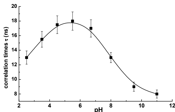
Fig. 2. Correlation times ( \tau ) as a function of pH for Tempo spin label in lyophilized cytochrome c.
