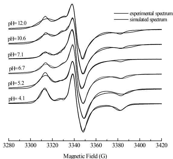
Fig. 1. Experimental and simulated spectrum of Tempo labelled cytochrome c.
