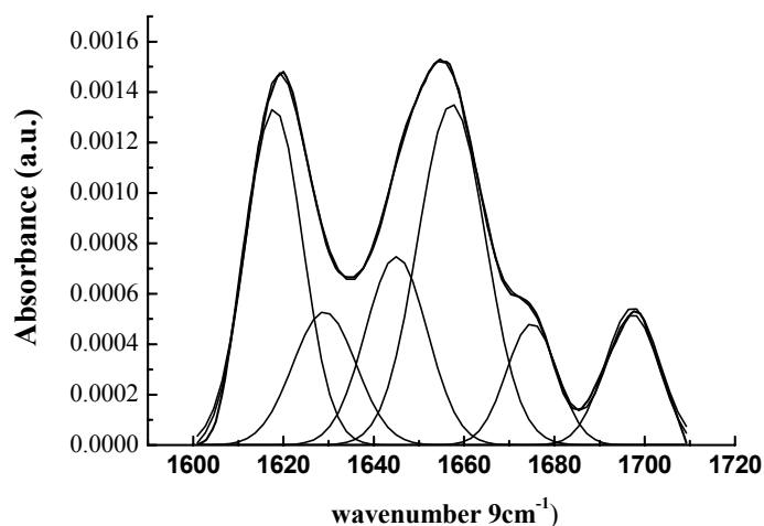
Fig. 3. The curve-fitted inverted second-derivative amide I spectrum of lyophilized cytochrome c at pH = 6.7. The inversion of second-derivative spectrum was done by factoring by -1 . The curve-fitting was carried out as described under Materials and Methods.
